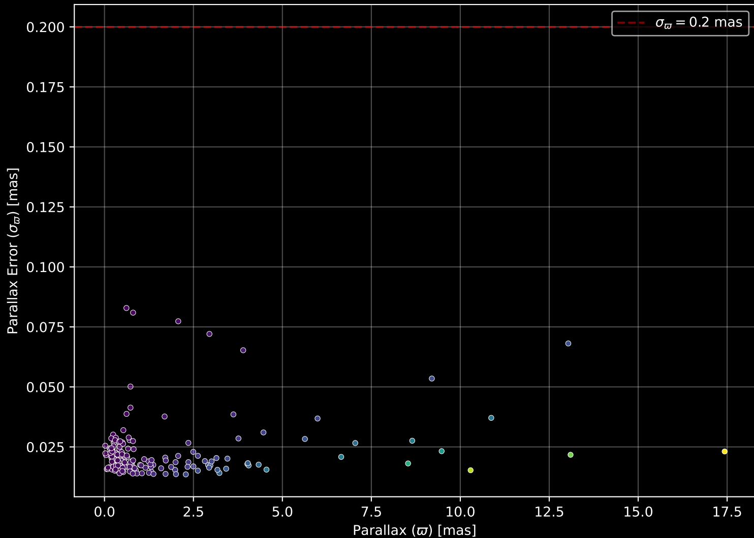
APOGEE DR17 Field: [075-45] Parallax Quality (n= 171)
