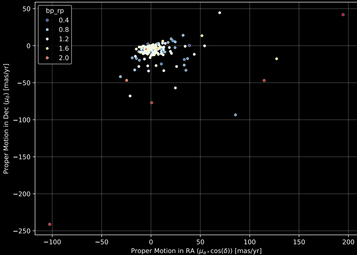
APOGEE DR17 Field: [075-45] Proper Motion Diagram (n= 171)
