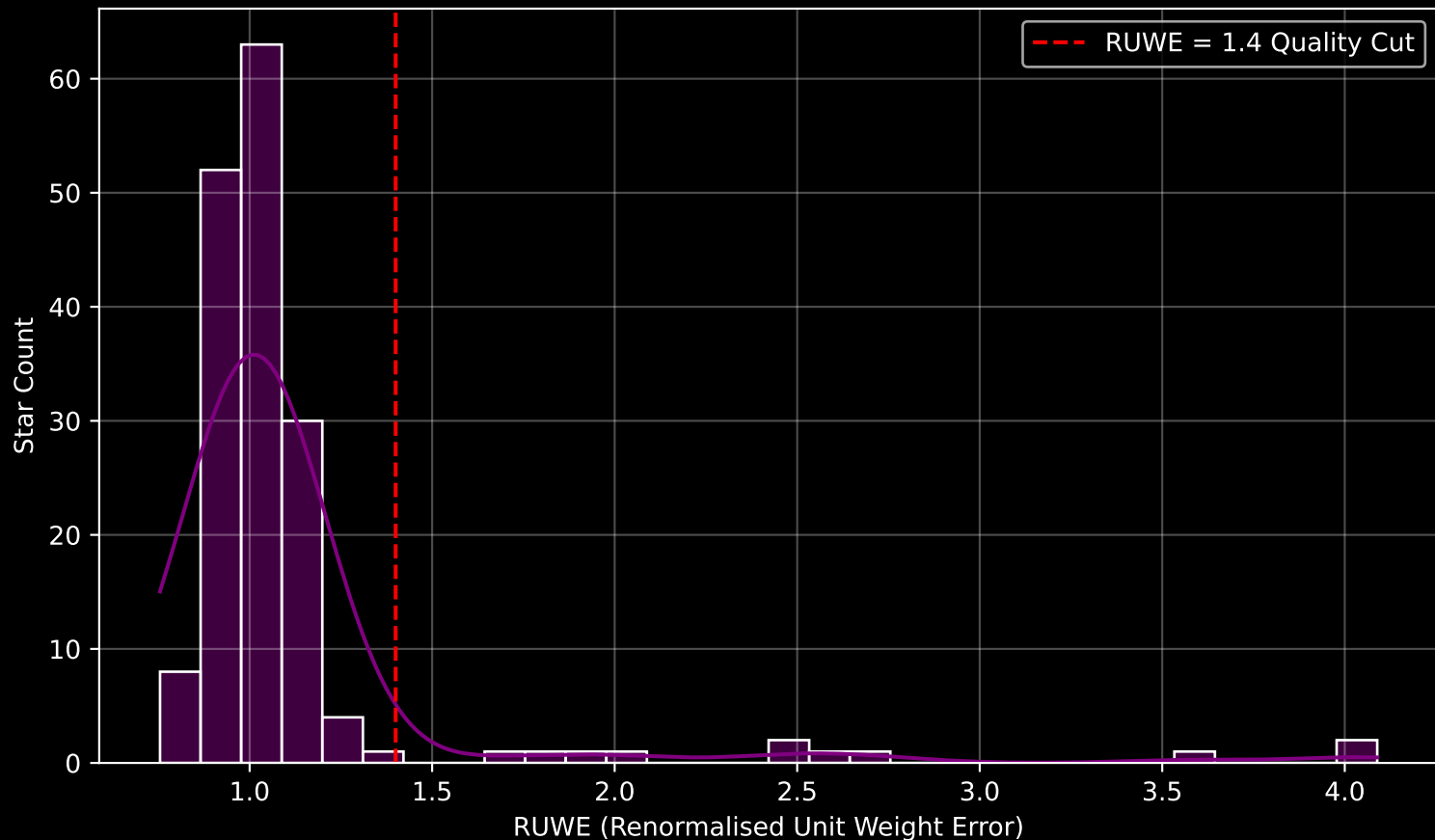
GAPOGEE DR17 Field [075-45] RUWE Distribution (n= 169)
