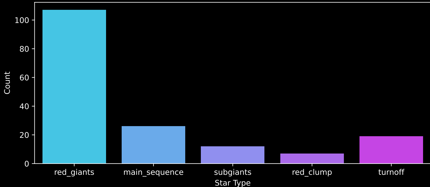
APOGEE DR17 Field: [075-45] Count plot of Star Type
