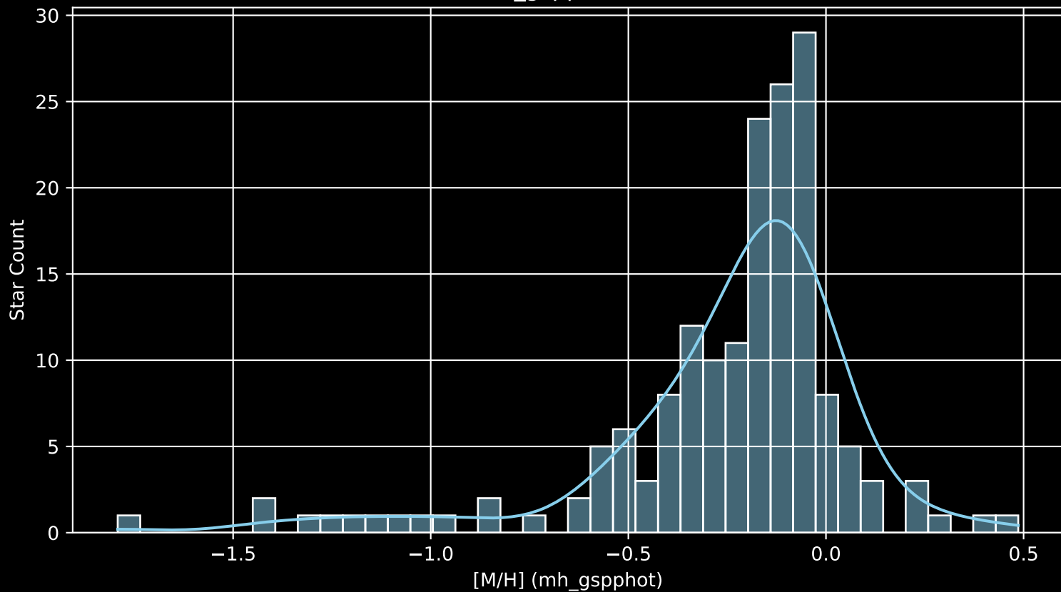
APOGEE DR17 Field: [075-45 [M/H] (mh_gspphot) (n= 171)
