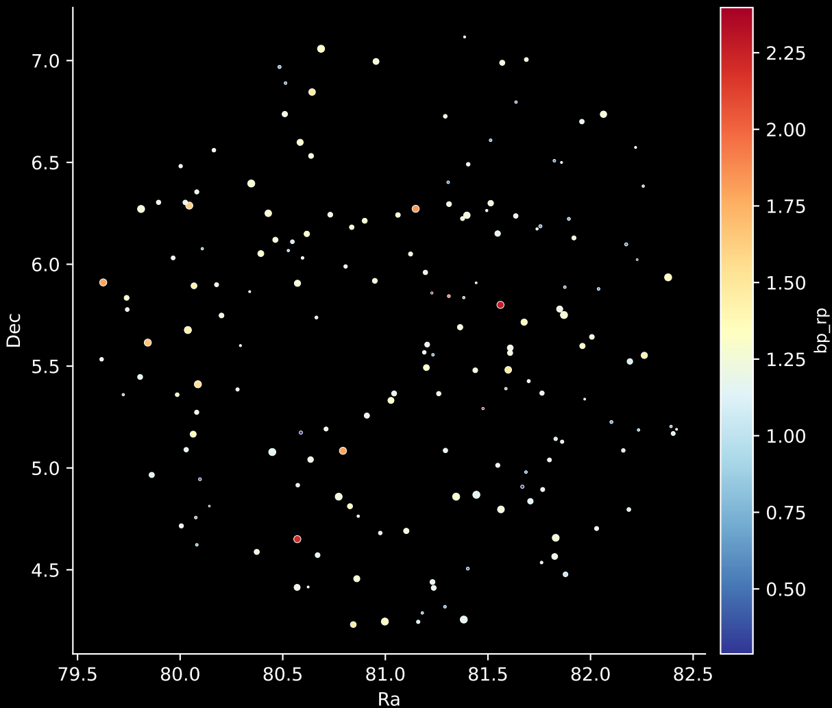
APOGEE DR17 Field: [075-45] Stars: 171
