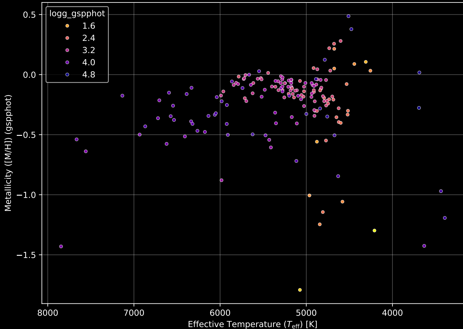
APOGEE DR17 Field: [075-45] Stellar Population Parameters (n= 171)
